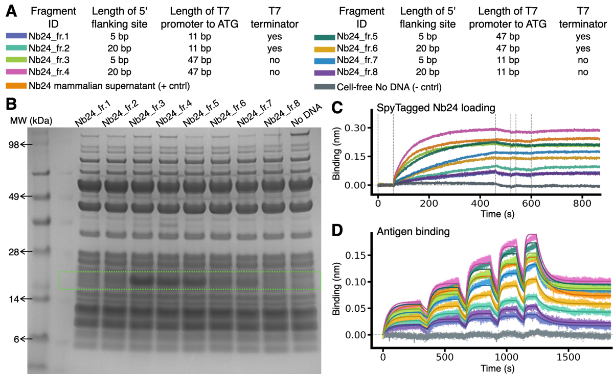
Figure S3. Optimisation of linear gene fragments for cell-free expression. (A) Table with the tested fragment IDs and their different spacer lengths. Colours correspond to the lines in the plots. Columns are the length of the 5' end of the fragment, the length of the region, which includes the ribosome-binding site, between the T7 promoter and the start codon (ATG), and the presence or absence of a T7 terminator. All DNA sequences are provided in Supplementary Dataset 1 . (B) SDS-PAGE with Instant Blue staining of the cell-free reactions after overnight expression from the different gene fragments (different wells), including a No DNA control, which is used to show the various component of the cell-free expression mixture when no protein is being expressed. An extra band is visible in some wells at just above 17 kDa (inside the green box, which serves as a guide for the eye) corresponding to nanobody Nb24 with a SpyTag003 and a 6xHis tag at its C-terminus (as in Fig. S1 ). The band is most apparent for fragments 3, 4, and 5. (C) BLI sensorgrams of the loading of the SpyTagged product to the biotinylated SpyCatcher003 already on the sensor. Sensorgrams have been aligned to the previous buffer step to highlight differences in loading rates, which correspond to differences in expression levels. The grey trace is the negative control showing that no loading is observed from the cell-free expression mixture not expressing a SpyTagged nanobody. The orange trace serves as a positive control and corresponds to SpyTagged Nb24 expressed in mammalian cells and loaded from the cells' supernatant. In agreement with the SDS-PAGE, Nb24 from fragments 3, 4 and 5 loads rather quickly and reaches plateau in less than 400 seconds, while Nb24 from all other fragments loads more slowly, denoting substantially lower expression levels. As expected, no loading is observed from the negative control. (D) BLI sensorgrams of the antigen binding steps, aligned to the assay baseline and fitted to a 1:1 partial dissociation binding model (solid lines, except for the negative control). The antigen – \beta_2 -microglobulin, used as analyte – was present at increasing concentrations of 25, 50, 100, 200, 400 nM in each association phase.
