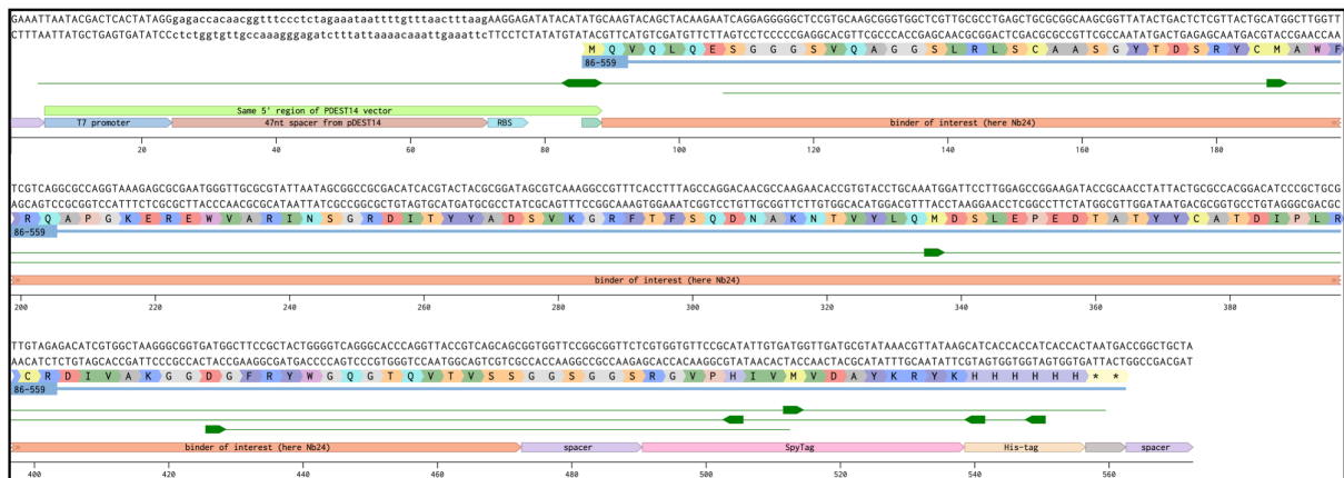
Figure S1. Sequence of linear DNA fragment used for cell-free expression. DNA sequence of the double-stranded linear DNA fragment optimised for cell-free expression. The coding sequence is also shown as translation. This example is for the Nb24 nanobody, but all other binders were obtained in the same way by substituting the binder sequence (orange annotation) with that of the binder of interest. The various annotations below the sequence describe what the relevant pieces are: RBS stands for ribosome binding site, and the His-tag at the C-terminus of the coding sequence is optional (it is not needed to run the SpyBLI assay, but it was present in the constructs used in this study, as it can be used for affinity-purification). We also provide a copy-paste friendly version of the above DNA sequence, with the parts encoding Nb24 and the 6xHis-tag in lower case, and start and stop codons in bold font:
