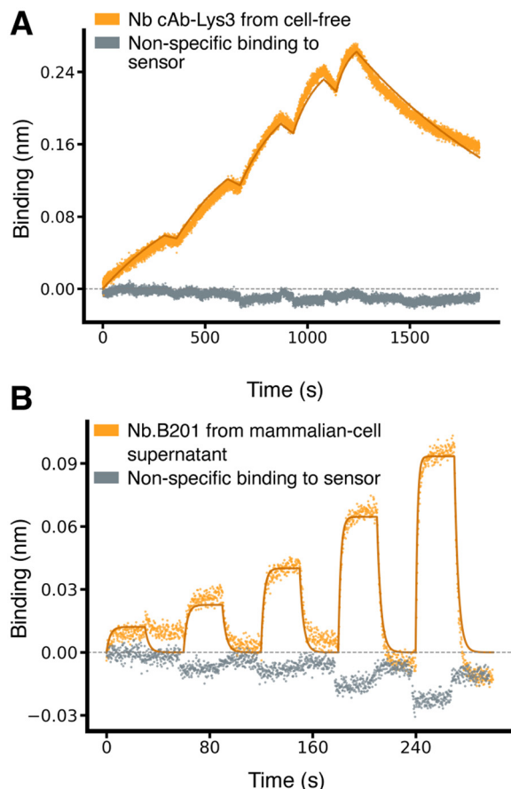
Fig. 3 Characterisation of nanobodies spanning a broad range of affinities. (A) Binding sensorgrams of SpyTagged nanobody cAb-Lys3 (PDB ID 1mel) loaded from cell-free-expression blend and binding to purified hen egg-white lysozyme, which was used as analyte at increasing concentrations of 0.625, 1.25, 2.5, 5, 10 nM. The solid lines correspond to a fit with a 1:1 standard binding model (fit RMSE \cong 0.007 nm, \cong 2.8% of the response window). (B) Binding sensorgram of SpyTagged nanobody Nb.B201 (PDB ID 5vnw) loaded from a mammalian-cell supernatant and binding to HSA, which was used as analyte at increasing concentrations of 62.5, 125, 250, 500, 1000 nM. The solid lines correspond to a fit with a 1:1 standard binding model (fit RMSE \cong 0.006 nm, \cong 6.4% of the response window).
