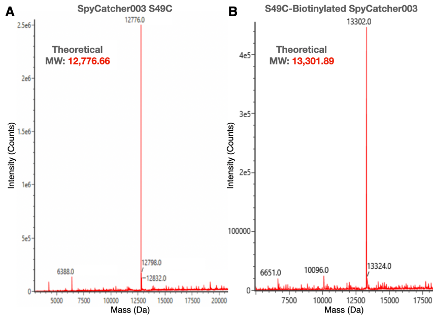
Figure S6. Deconvoluted liquid-chromatography mass spectrometry spectra (electrospray ionization) of purified SpyCatcher003 S49C following TEV cleavage ( A ), and of the same protein after maleimide biotinylation ( B ). Expected, theoretical molecular weights (MW) calculated from the amino acid sequence and the maleimide-PEG2-biotin (525.23 Da) are also reported on the panels.
