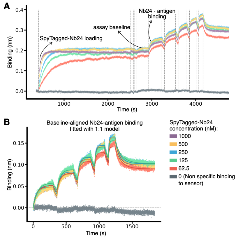
Figure S2. Robustness of kinetic measurements across a more than 10-fold variation in loading concentration. (A) BLI sensorgrams resulting from the loading of different concentration of SEC-purified SpyTagged Nb24 (see legend) onto sensors pre-loaded with biotinylated SpyCatcher003 and then probing the same wells as detailed in Fig. 1 of the main text. (B) Fits carried out with a 1:1 partial dissociation binding model (solid lines) of the analyte ( \beta_2 microglobulin) associations and dissociations steps. Traces are aligned to the assay baseline, and the antigen concentrations were 25, 50, 100, 200, and 400 nM.
