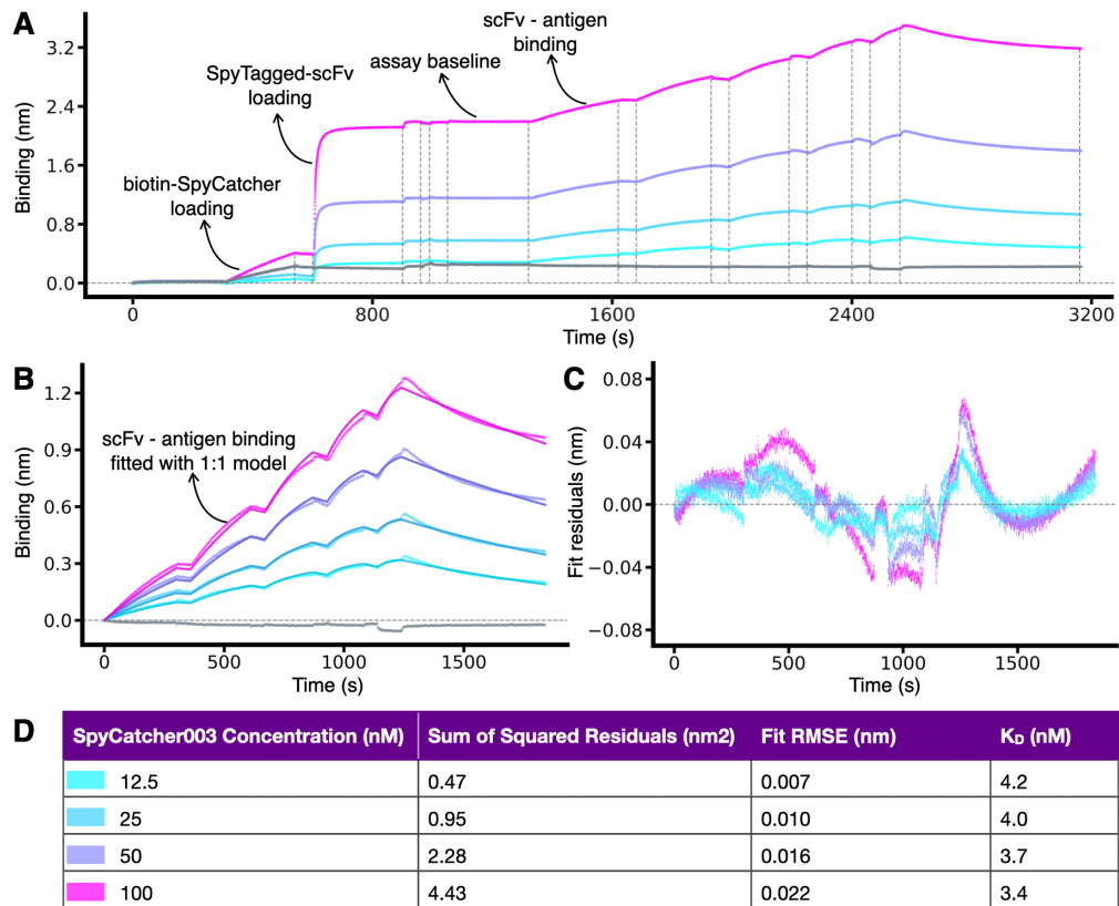
Figure S7. Optimisation of sensor crowdedness for optimal signal quality. In BLI, the more ligand is loaded the higher the signal to noise ratio is obtained. However, excessive loading leads to large deviations from the theoretical binding models used to fit the data, due to artifacts resulting from surface heterogeneity or mass transport. (A) BLI sensorgrams resulting from the loading of different concentration of biotinylated SpyCatcher003 (see legend in D ) on the streptavidin sensors, and then probing the same wells as detailed in Fig. 1 of the main text. In all panels, the ligand is always the same anti-CD16a scFv loaded from mammalian-cell supernatant, and the analyte is always the same concentration series of monovalent CD16a (increasing concentrations of 6.25, 12.5, 25, 50, 100 nM). The control for non-specific binding of the analyte (grey trace) was loaded with 50 nM SpyCatcher003, but then not loaded with any SpyTagged protein but blocked with free SpyTag003 peptide in the blocking step (see Fig. 1 ). (B) Fits carried out with a 1:1 standard binding model (solid lines) of the analyte associations and dissociations steps. (C) Residuals plot of the fits in B . (D) Table with the different SpyCatcher003 concentrations used at the loading steps, the sum of the squared residuals for the fits, the fit root-mean-squared error (RMSE), and the resulting K D . The data show that, while all traces yield very similar K D well within the reproducibility of the technique, the trace obtained with the lowest SpyCatcher003 concentration of 12.5 nM has the best agreement with the theoretical binding model, as shown by the residual plot, the fit RMSE, and the sum of squared residuals.
